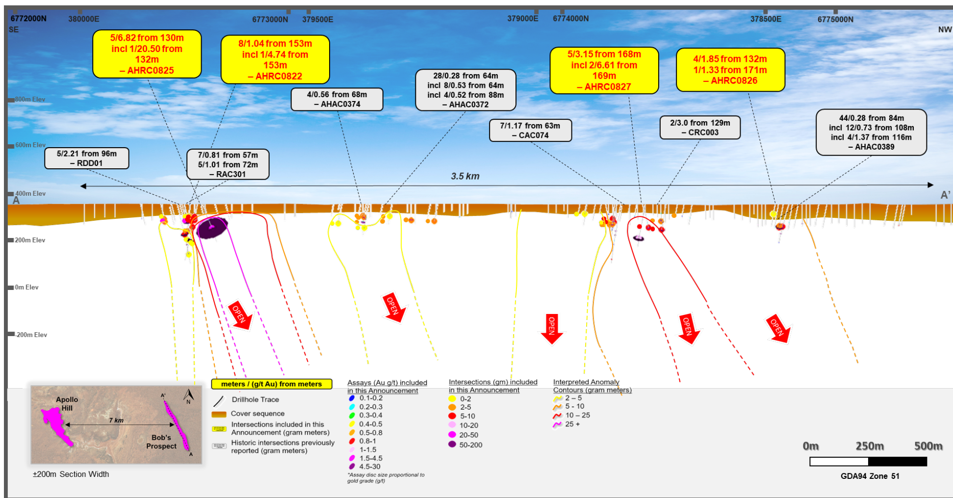
Figure 1 – Simplified geological long-cross section A-A1 of recent drill results – higher grade gold vectors apparent.
