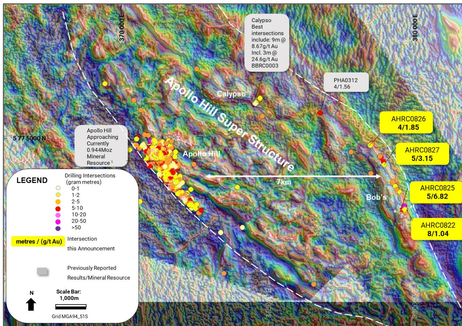
Figure 2 – Plan view of the current mineralisation footprint across the Apollo Hill camp with new results highlighted – merged aeromagnetic and gravity geophysics back-ground highlights the geological complexity and multiple exploration targets at the ‘Camp Scale’; location of Figure 3 cross section a-a1 highlighted on diagram.
