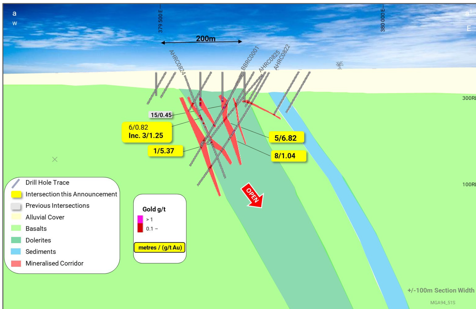
Figure 3 – Geological cross section – a-a1 of Bob's Prospect; wide mineralised corridor and multiple stacked lodes noted; location of cross section a-a1 illustrated on Figure 2.
