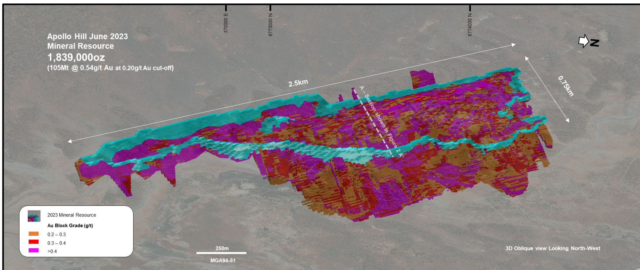
Figure 1 – Oblique view 3D Representation of the June 2023 Apollo Hill Mineral Resource model and selected nominal constraining pit for reporting, shown with topography – Mineral Resource reported within/above the pit shell only.
