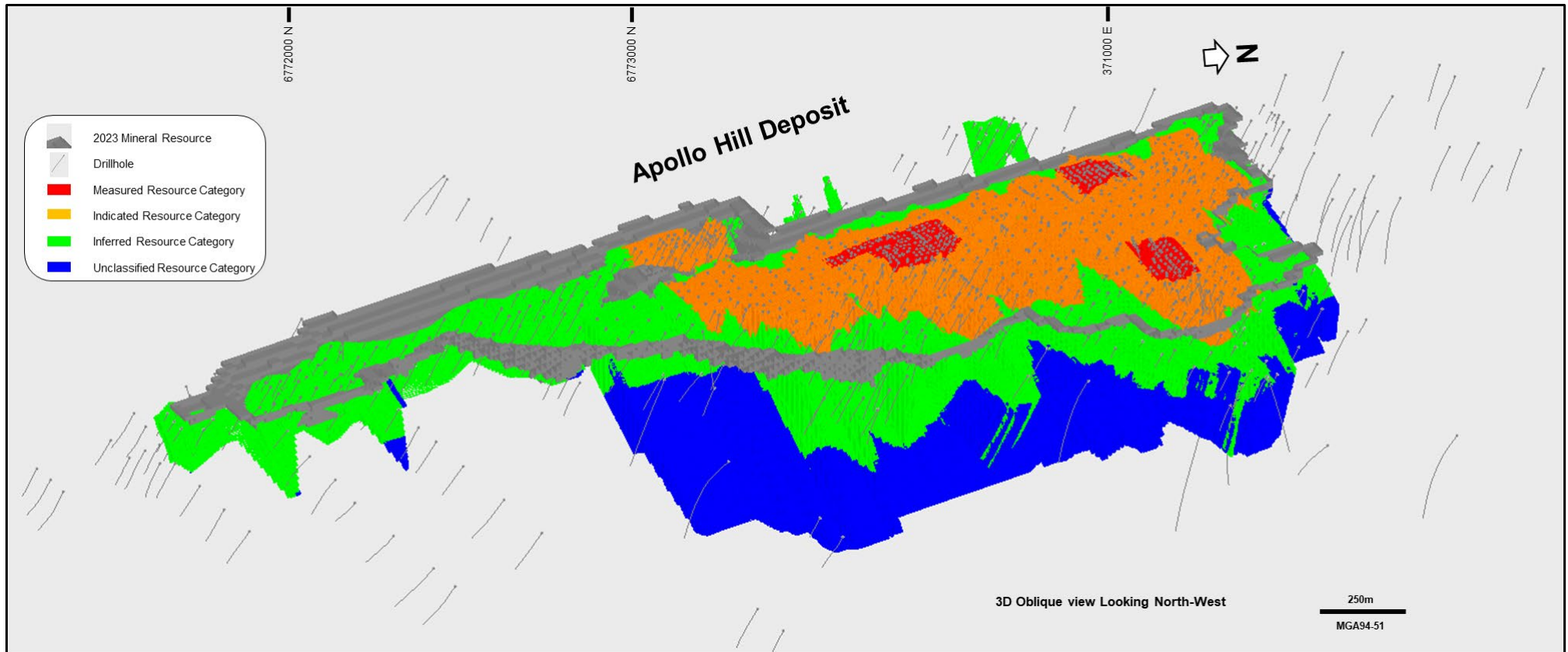
Figure 3 – Measured, Indicated and Inferred Mineral Resource Classifications relative to the nominal constraining open pit shell. Material outside of the nominal pit shell is not reported.
