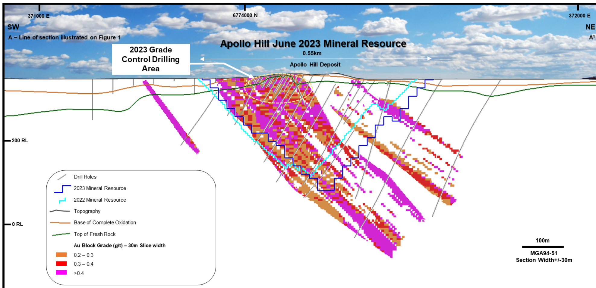
Figure 2 – Oblique block model cross-section (South West – North East, A-A 1 on Figure 1 3D diagram) +/-30 m showing gold grade and block locations.
