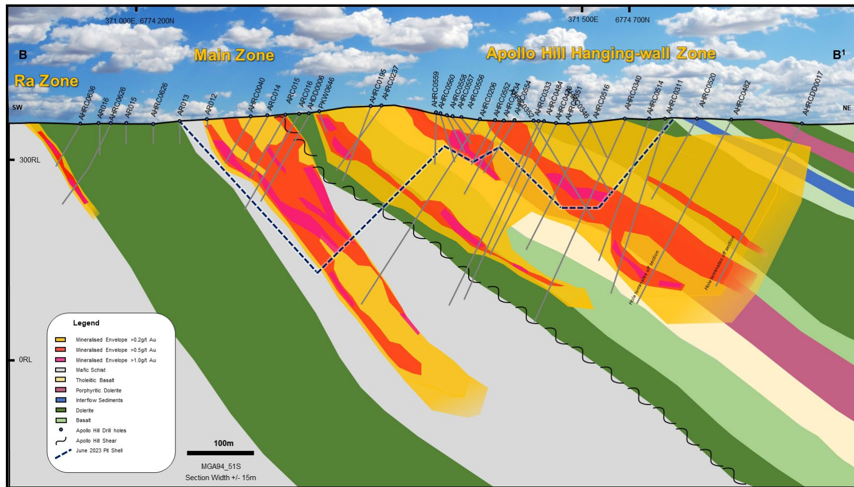
Figure 7 – Apollo Hill Shear Zone and gold mineralisation in southwest-northeast cross section (+/- 15m) B-B¹ location illustrated in plan view Figure 6.
