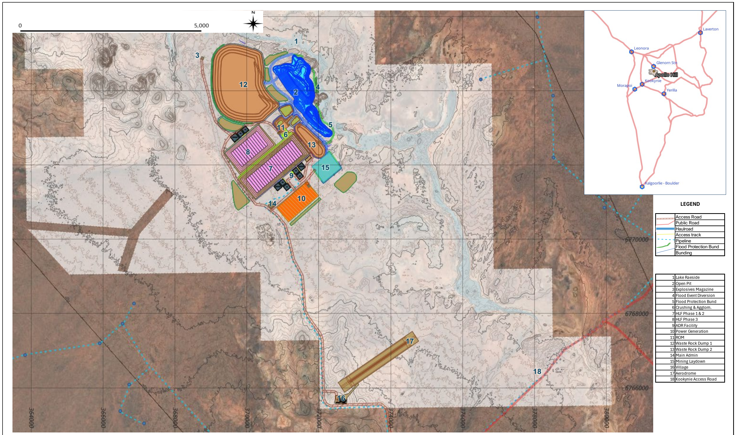
Figure 11.3: Apollo Hill Overall Site Plan.
