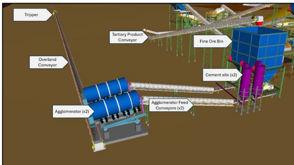
Figure 5.5: Agglomeration Circuit.
