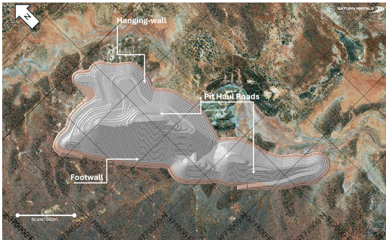
Figure 3.4: Plan View of Apollo Hill PFS Final Pit Design.
