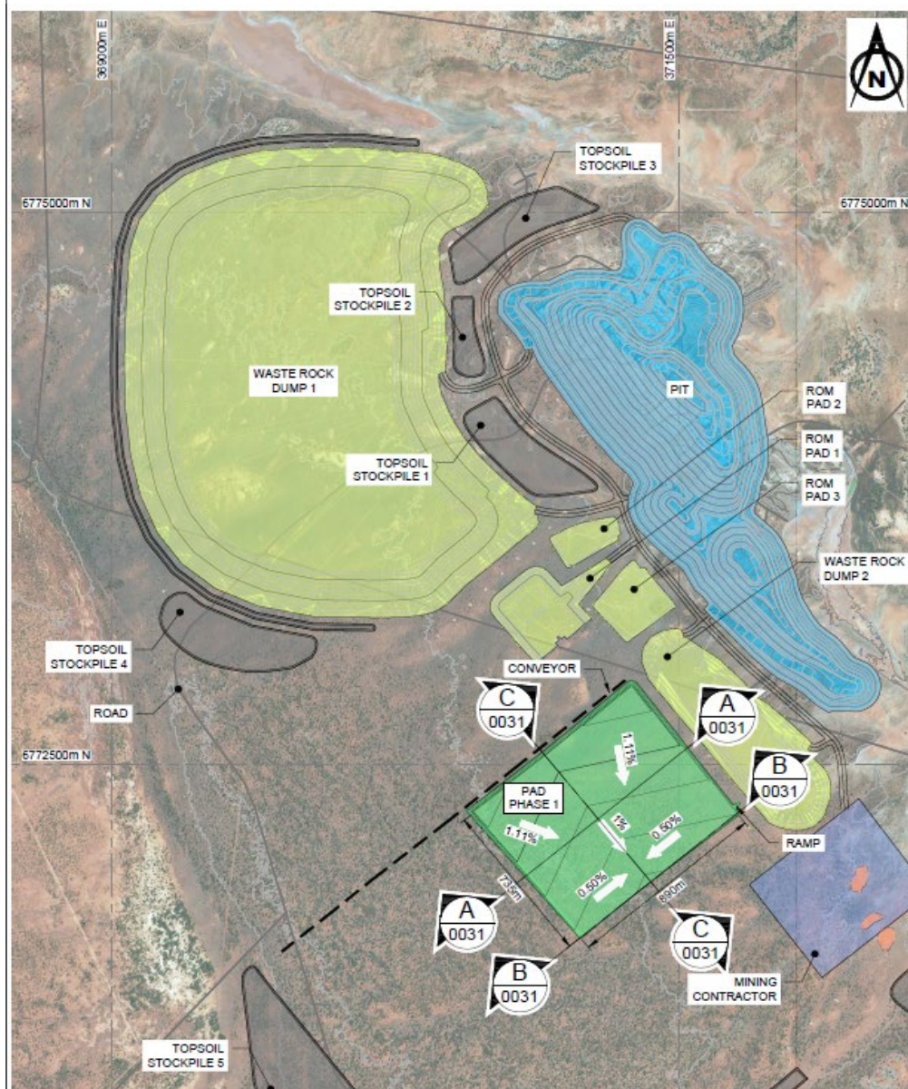
PAD BASE LAYOUT - PHASE 1 SCALE 1:15,000
