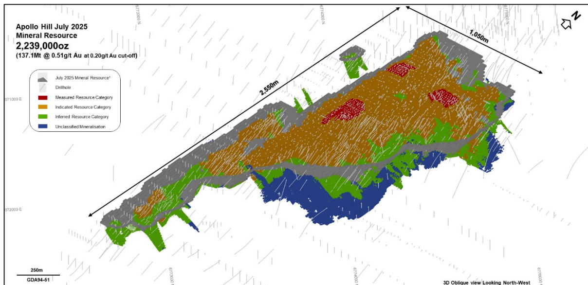
Figure 2.7: Measured, Indicated, Inferred Mineral Resource and Unclassified Mineralisation Relative to the Nominal Constraining Open Pit Shell. Blocks Illustrated are >0.20 g/t Au (cut-off grade). Material Outside of the Nominal Pit Shell and Material Left as Unclassified is Not Reported.
